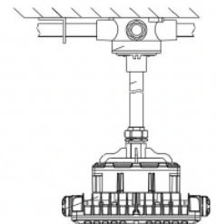
Suspended installation
