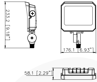
Knuckle
