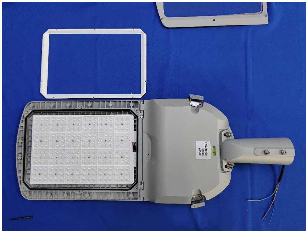
Figure 11.: Internal view of model MSL-F300
