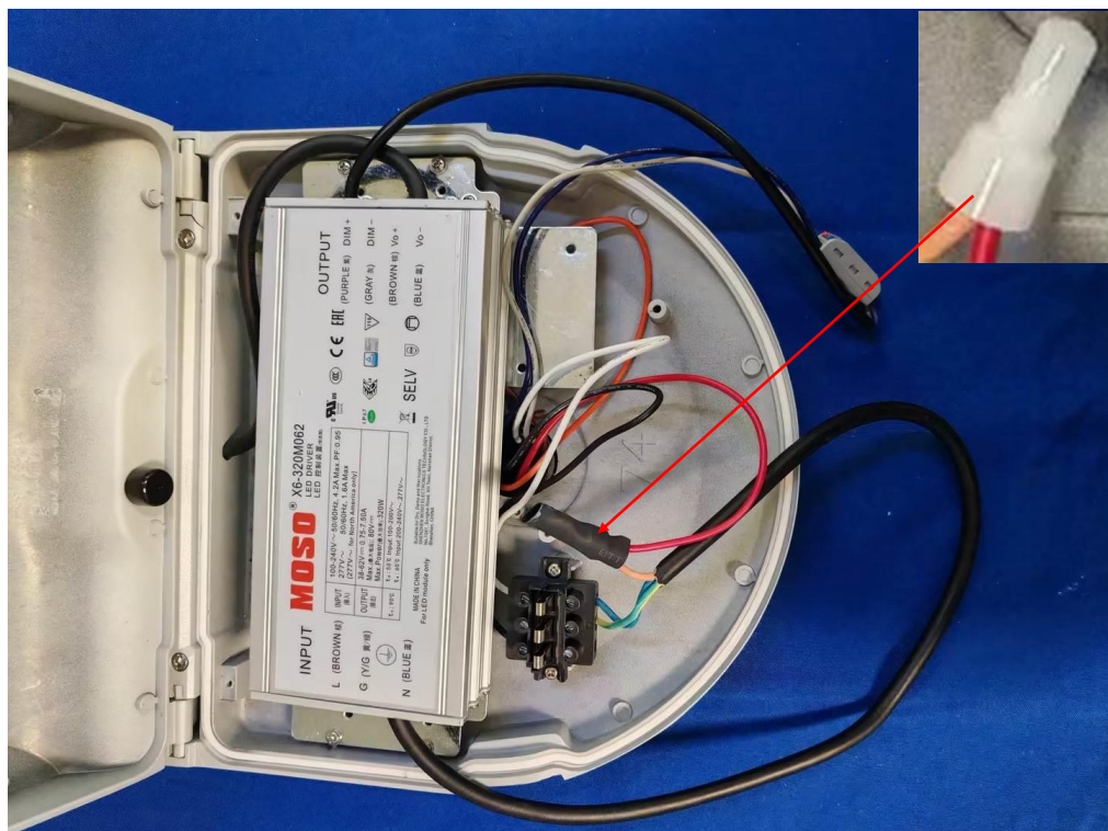
Figure 8.: Internal view of model MSL-F300
